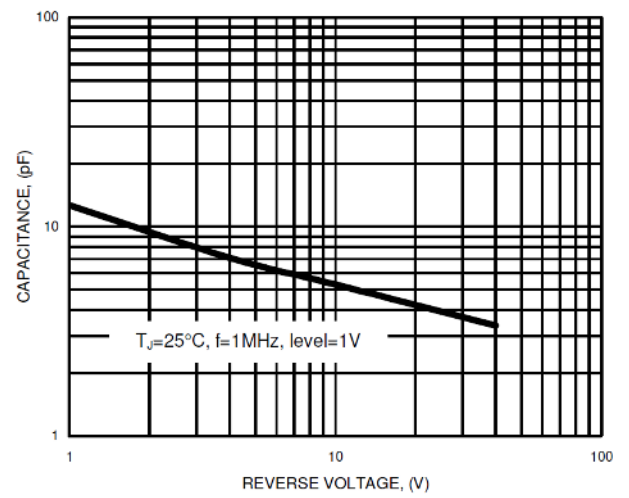
FIG.4- TYPICAL TOTAL CAPACITANCE
