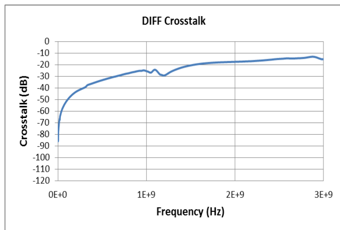
Figure 21. DIFF Crosstalk
