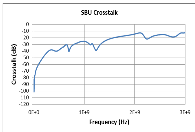
Figure 21. SBU Crosstalk
