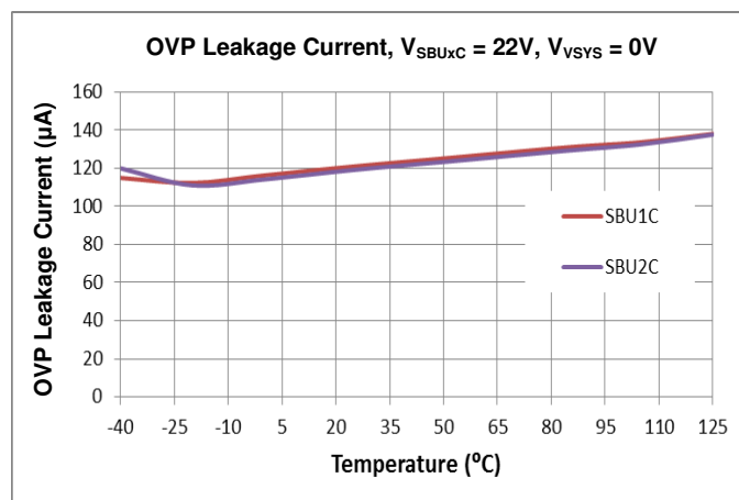
Figure 8. SBUx 22V OVP Leakage Current vs. Temperature
