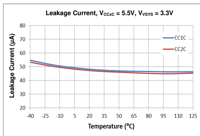
Figure 6. CCx Leakage Current vs. Temperature
