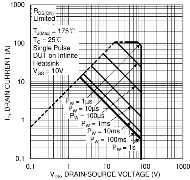
Fig. 13 SOA, Safe Operation Area
