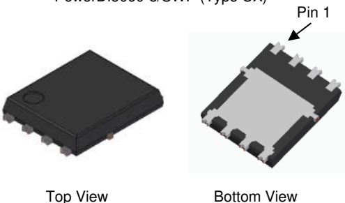
PowerDI5060-8/SWP (Type UX)
