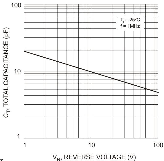
Fig. 4 Typical Total Capacitance vs Reverse Voltage
