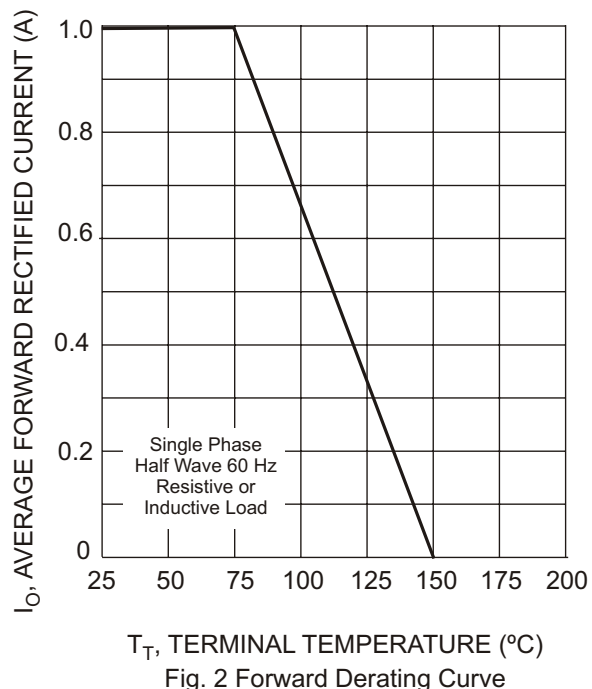
Fig. 2 Forward Derating Curve
