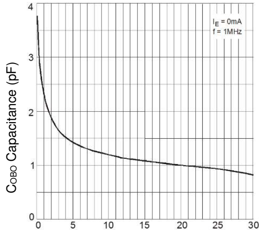
Fig.26 Typical C_{OBO} vs. V_R
