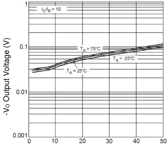
Fig.24 Typical V_O vs. I_O
