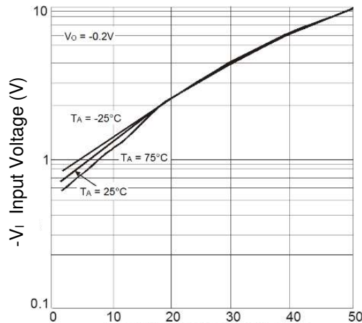
Fig.28 Typical V_I vs. I_O
