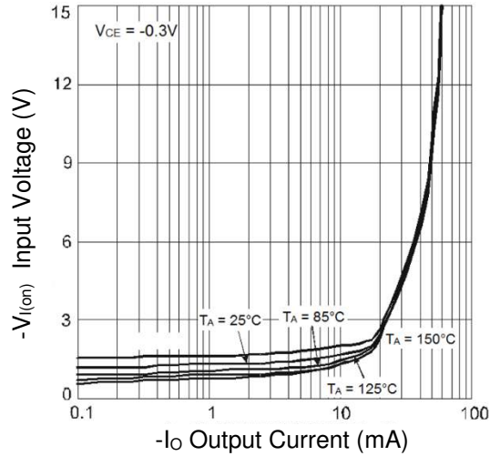
- I_O Output Current (mA) Fig.15 Typical V_I vs. I_O
