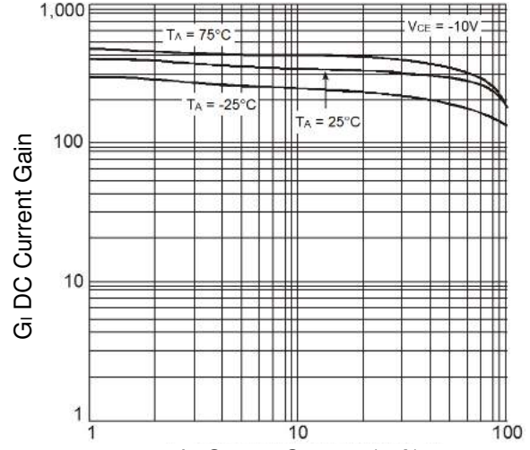
Fig.25 Typical G_I vs. I_O
