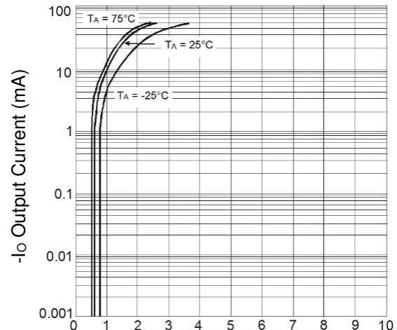
Fig.27 Typical I_O vs. V_I
