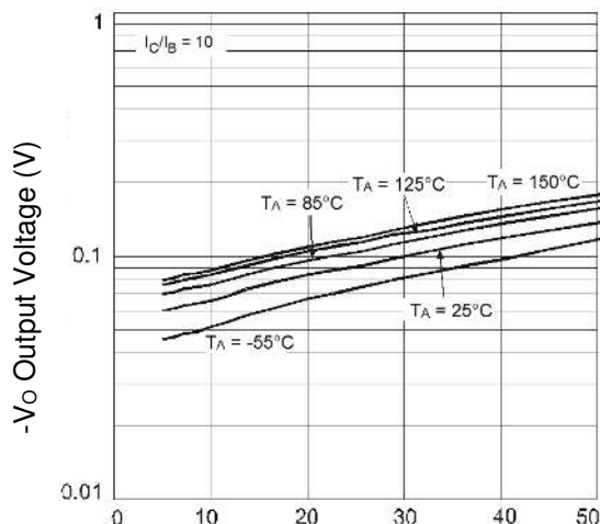
- I_O Output Current (mA) Fig.14 Typical V_O vs. I_O
