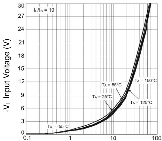
- I_O Output Current (mA) Fig.16 Typical V_I vs. I_O
