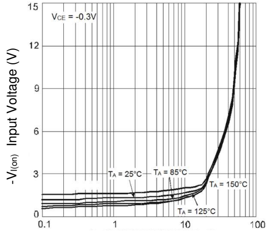
- I_O Output Current (mA) Fig.17 Typical V_{I(on)} vs. I_O
