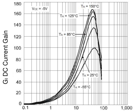
- I_O Output Current (mA) Fig.13 Typical G_I vs. I_O
