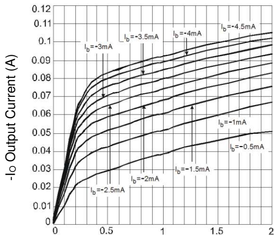
- V_O Output Voltage (V) Fig.12 Typical I_O vs. V_O
