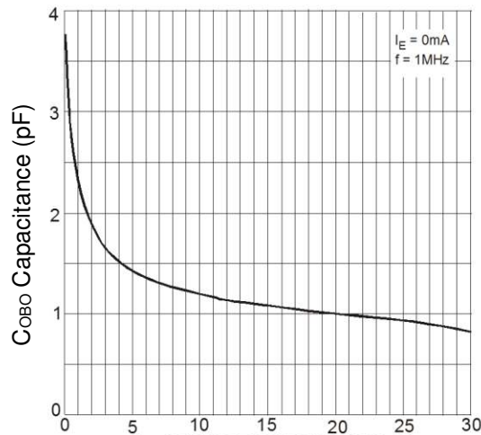
Fig.31 Typical C_{OBO} vs. V_R
