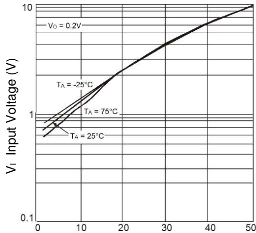
Fig.33 Typical V_I vs. I_O
