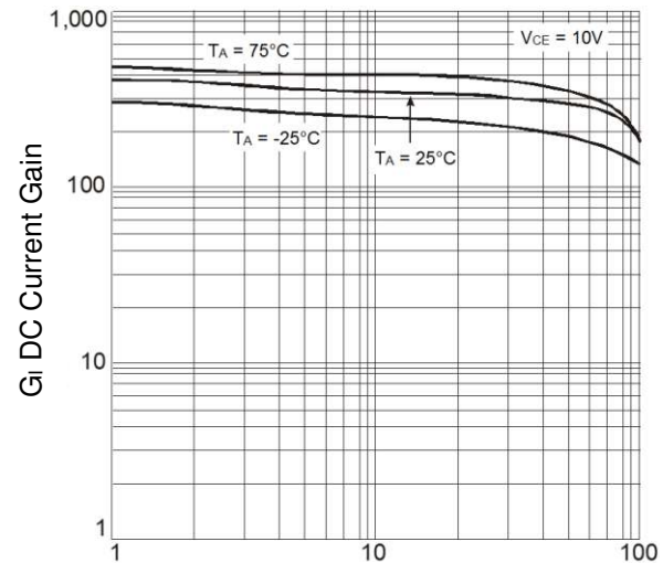
Fig.30 Typical G_I vs. I_O
