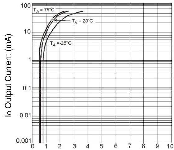
Fig.32 Typical I_O vs. V_I
