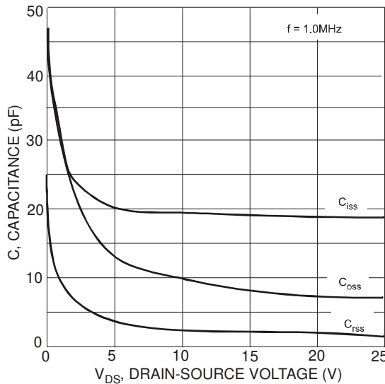
Fig. 5 Typical Capacitance
