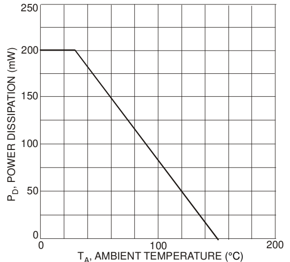
Fig. 6 Power Derating Curve, Total Package
