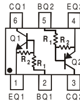
Device Schematic
