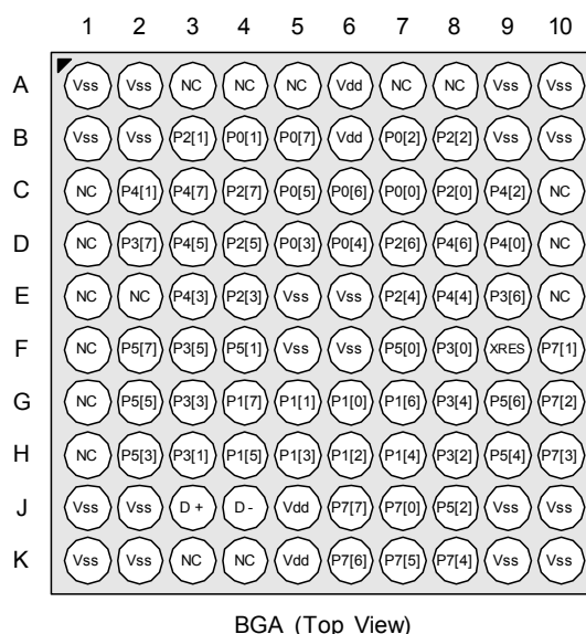
BGA (Top View)
