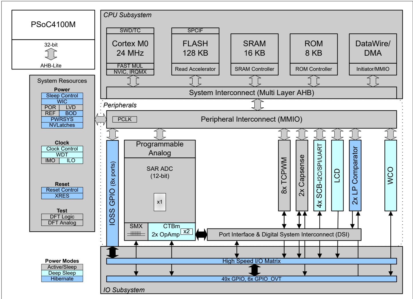
Figure 2 Block diagram
