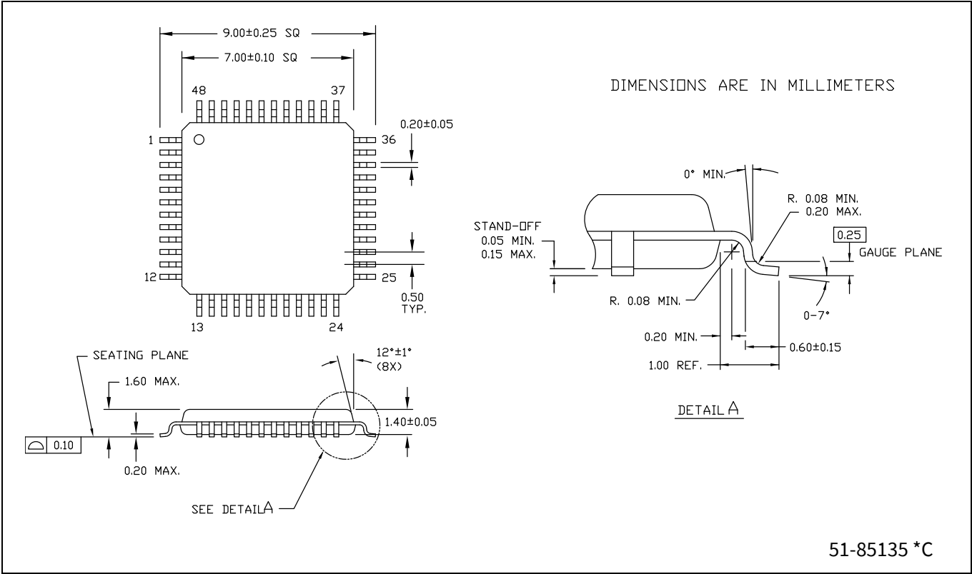
Figure 6 48LD TQFP 7x7x1.4 mm A48, PACKAGE OUTLINE, (PG-TQFP-48)
