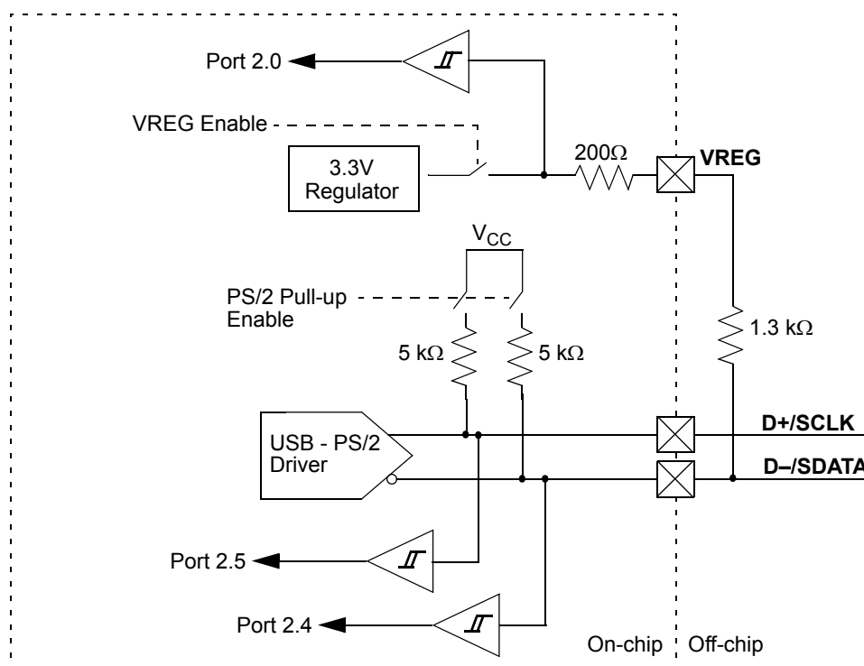
Figure 16-1. Diagram of USB - PS/2 System Connections
