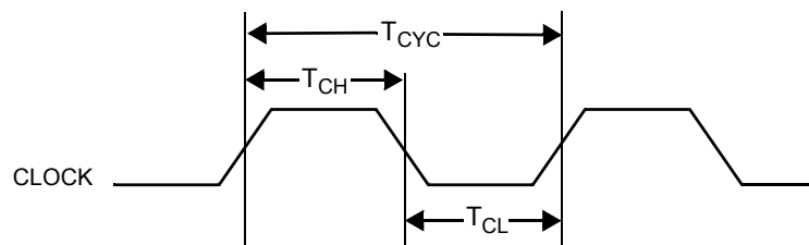
Figure 24-1. Clock Timing
