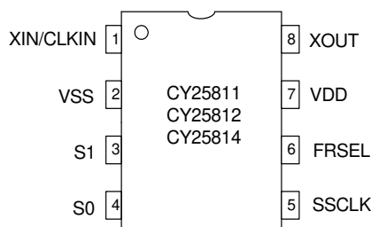
Figure 1. Pin Configuration – 8 Pin SOIC/TSSOP
