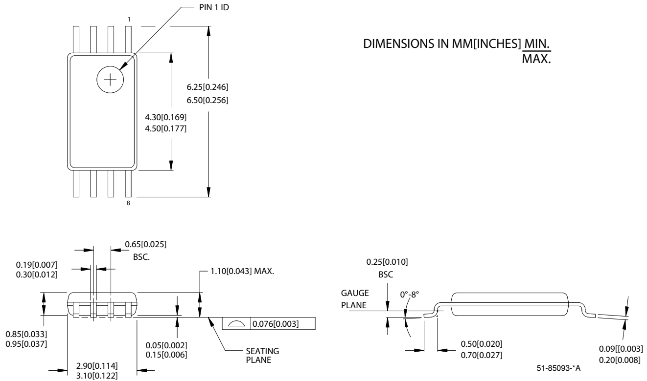
Figure 6. 8-Pin Thin Shrink Small Outline Package (4.40 MM Body) Z8
