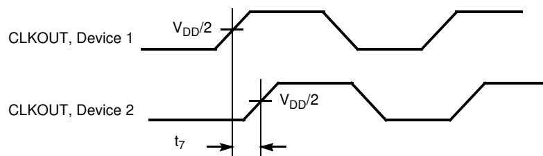
Figure 8. Device-Device Skew
