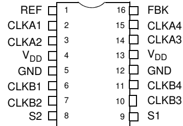
Figure 1. Pin Diagram - 16 Pin SOIC (Top view)
