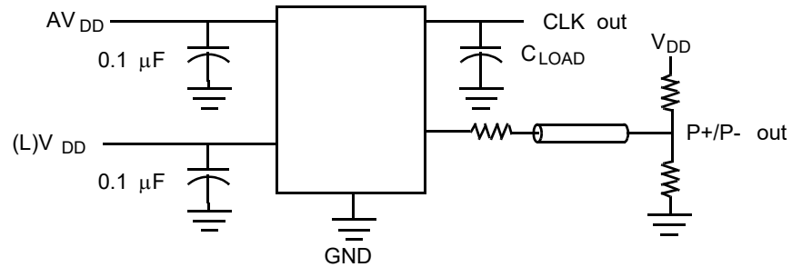
Figure 12. Test Circuit
