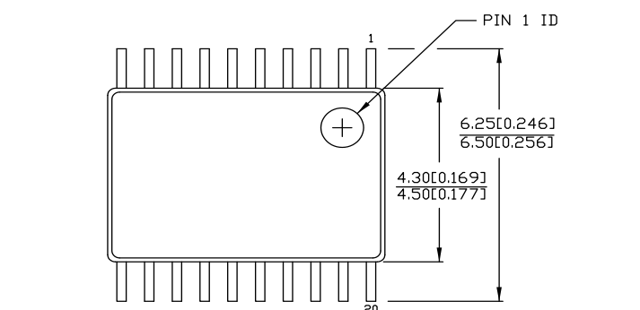
Figure 11. 20-pin TSSOP (4.40 mm Body) Package Outline, 51-85118
