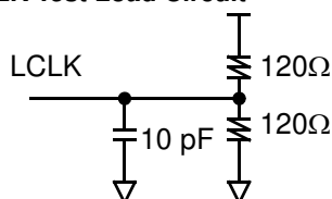
Figure 2. LCLK Test Load Circuit
