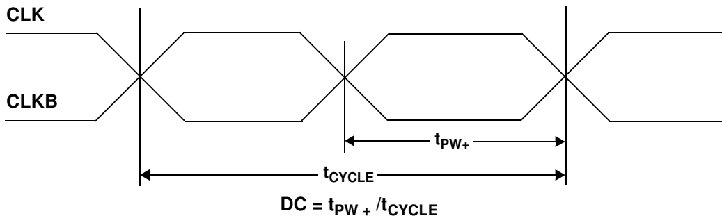
Figure 8. Duty Cycle
