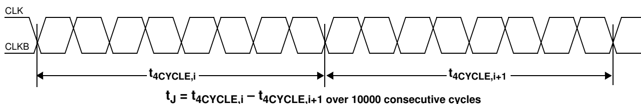
Figure 11. Short-Term Jitter
