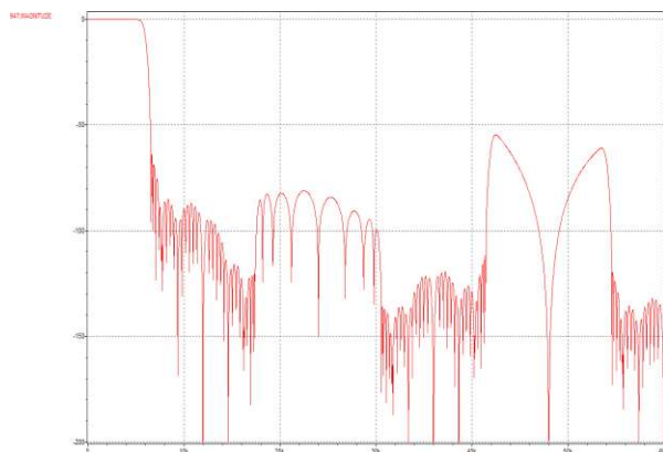
Figure 57 DAC Filter Response ( f_s=12\text{kHz} )
