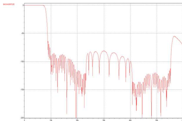
Figure 58 DAC Filter Response ( f_s=16\text{kHz} )
