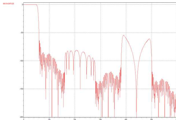
Figure 56 DAC Filter Response ( f_s=11.025\text{kHz} )
