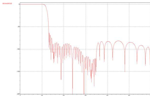
Figure 58 DAC Filter Response ( f_s=16\text{kHz} )
