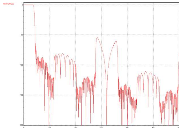
Figure 55 DAC Filter Response ( f_s=8\text{kHz} )
