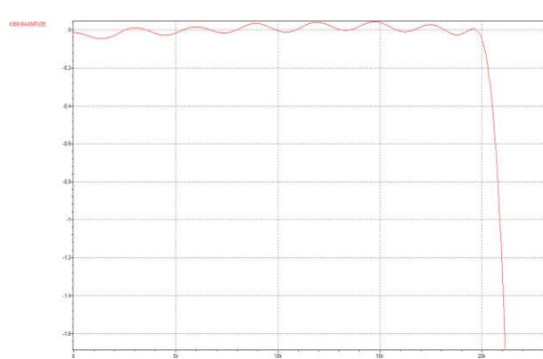
Figure 66 DAC Filter Passband Ripple ( f_s=44.1\text{kHz} )
