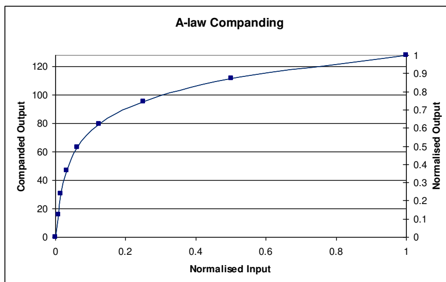
Figure 52 A-Law Companding
