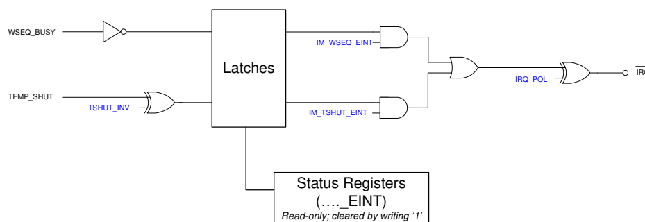
Figure 54 Interrupt Controller
