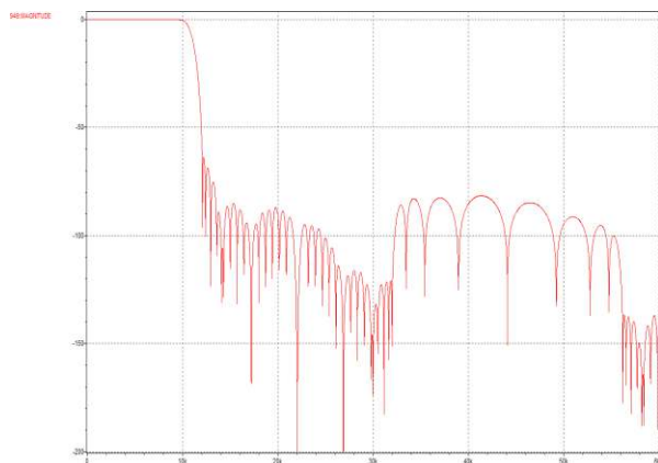
Figure 59 DAC Filter Response ( f_s=22.05\text{kHz} )
