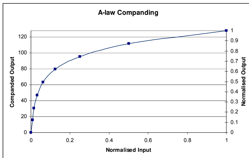
Figure 33 A-Law Companding
