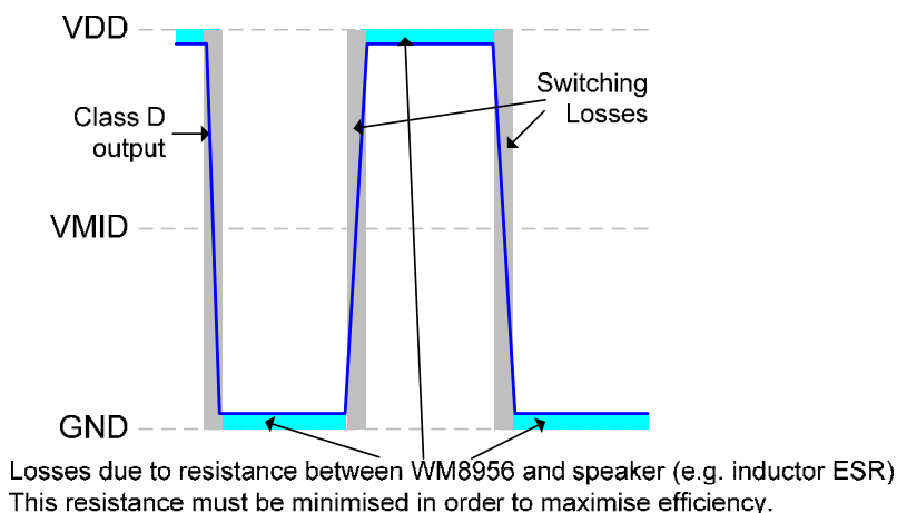
Figure 47 Speaker Connection Losses
