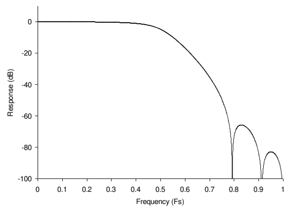
Figure 29 DAC Digital Filter Frequency Response – 128fs and 192fs Clock Modes
