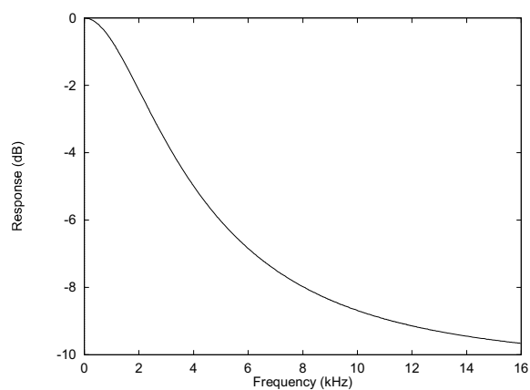
Figure 12 De-Emphasis Frequency Response (32kHz)
