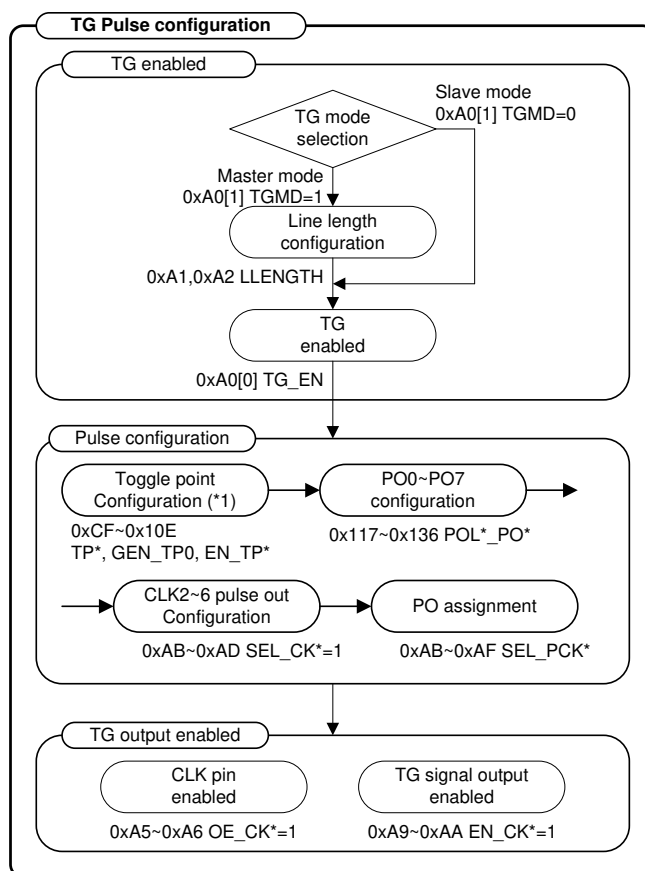
Figure 46 TG Pulse Configuration
