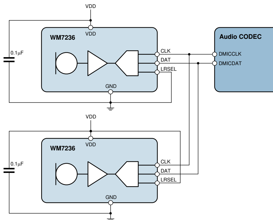
Figure 2 Stereo WM7236 Digital Microphone Connection
