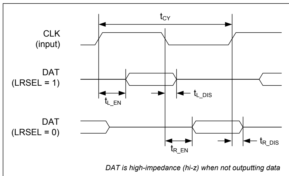
Figure 1 Digital Microphone Interface Timing
