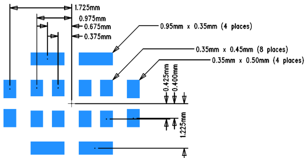
Figure 4 DM096 - Paste Stencil Pattern, Top View
