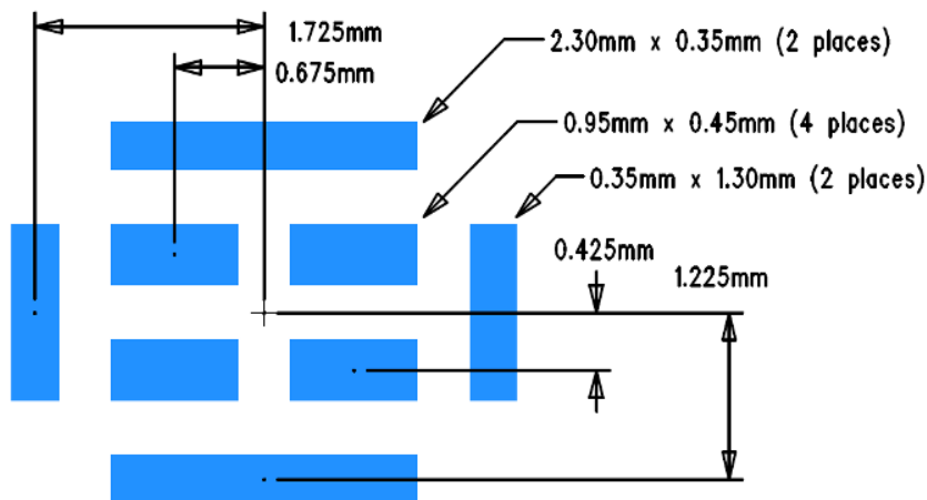
Figure 3 DM096 - PCB Land Pattern, Top View
