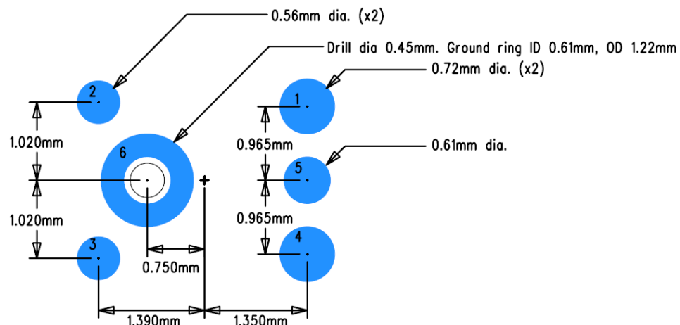
Figure 4 DM88 - PCB Land Pattern, Top View
