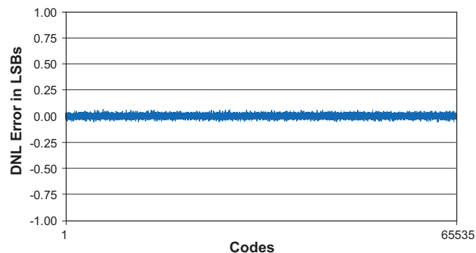
Figure 9. CS5571 DNL Plot
