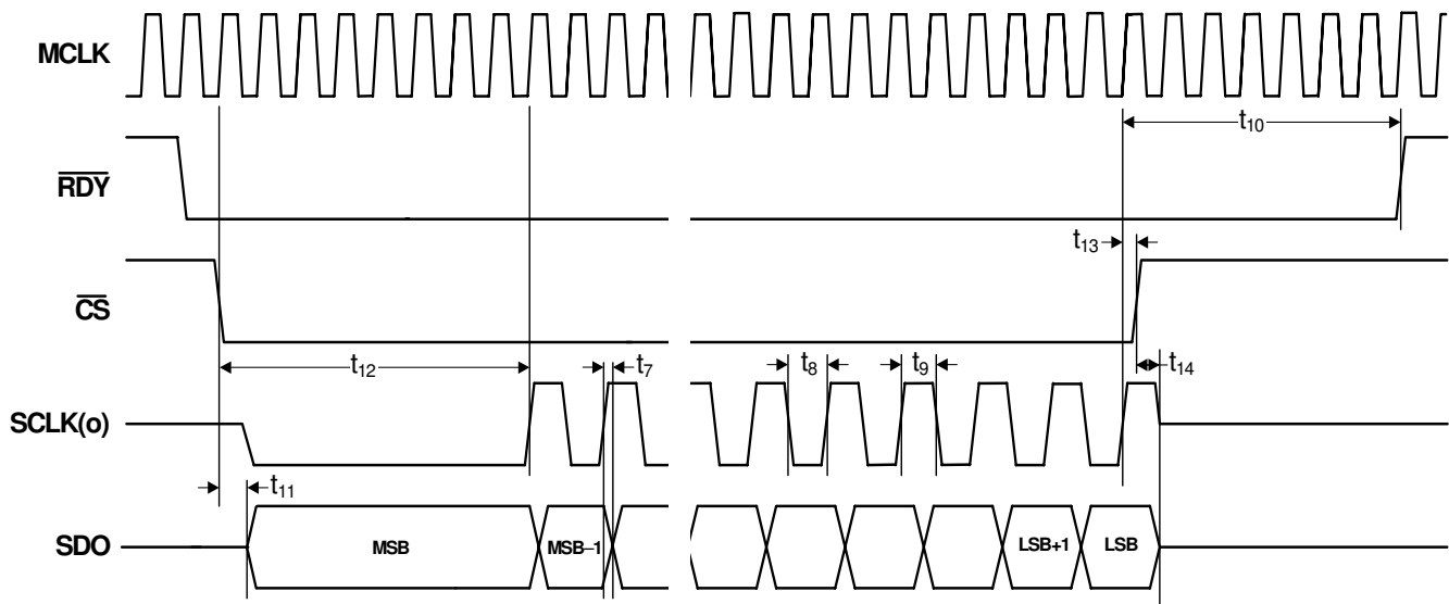
Figure 3. SSC Mode - Read Timing, \overline{CS} falling after \overline{RDY} falls (Not to Scale)
