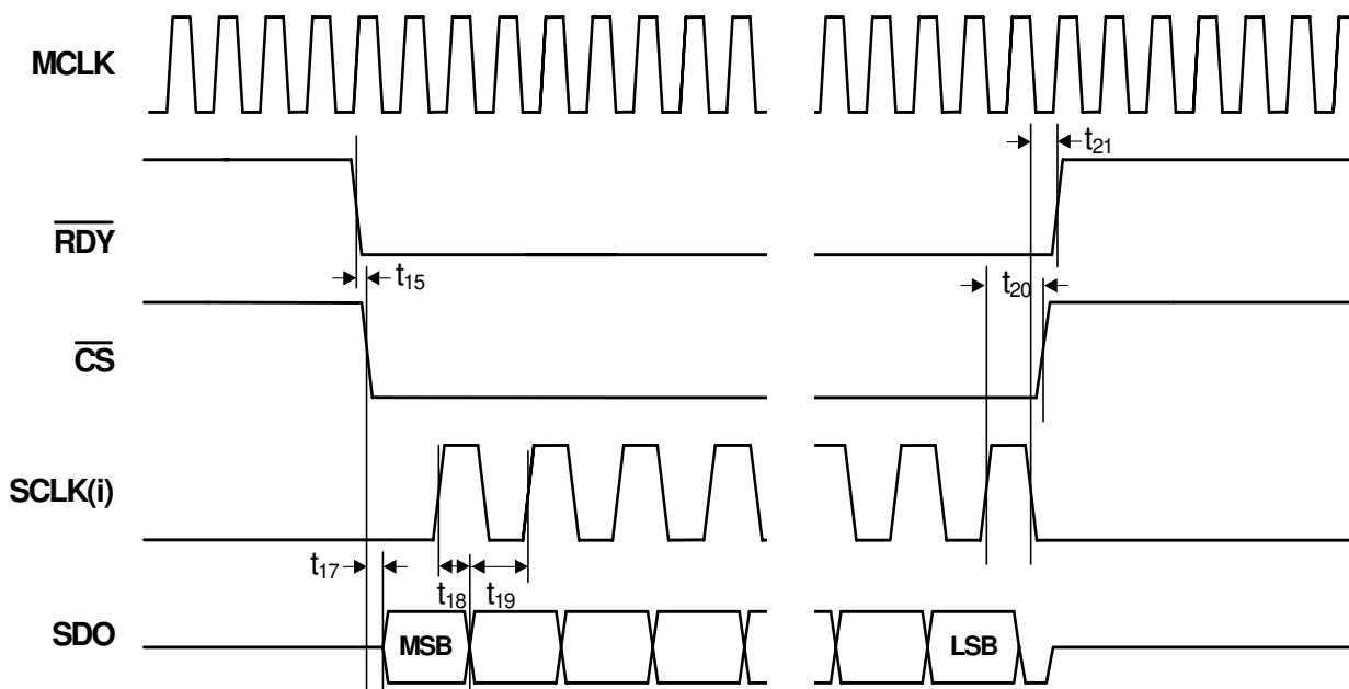
Figure 4. SEC Mode - Discontinuous SCLK Read Timing (Not to Scale)
