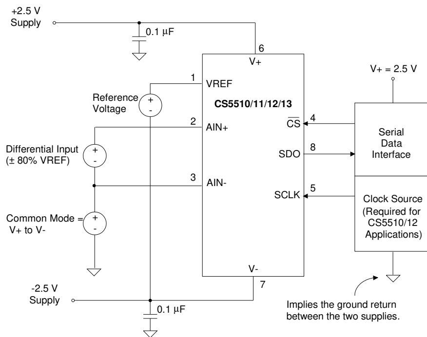
Figure 7. CS5510/11/12/13 Configured with \pm 2.5 V Analog Supplies.
