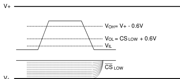
Figure 10. SDO Digital Output Levels.
