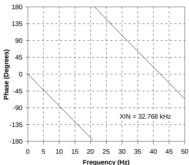
Figure 8. Filter Phase Plot to 50 Hz
