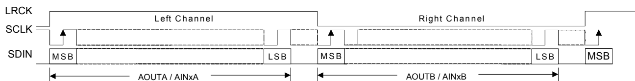
Figure 16. Left-Justified Format
