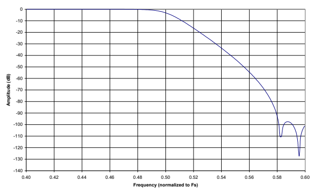
Figure 2. Single-Speed Mode Transition Band
