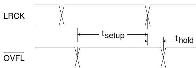
Figure 17. \overline{\text{OVFL}} Output Timing
