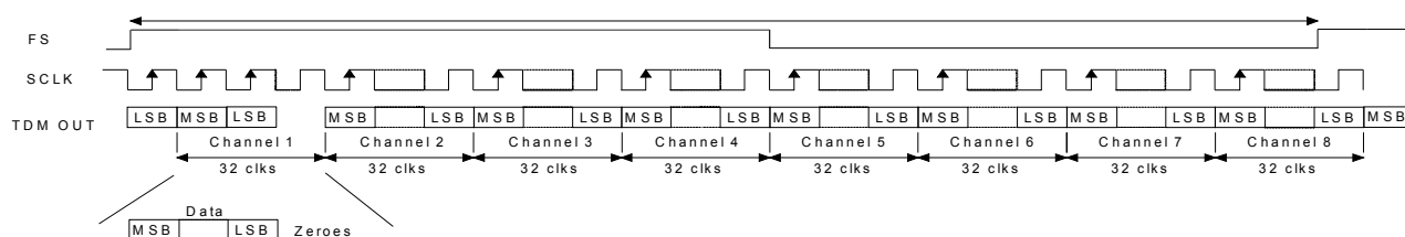
Figure 12. TDM Format
