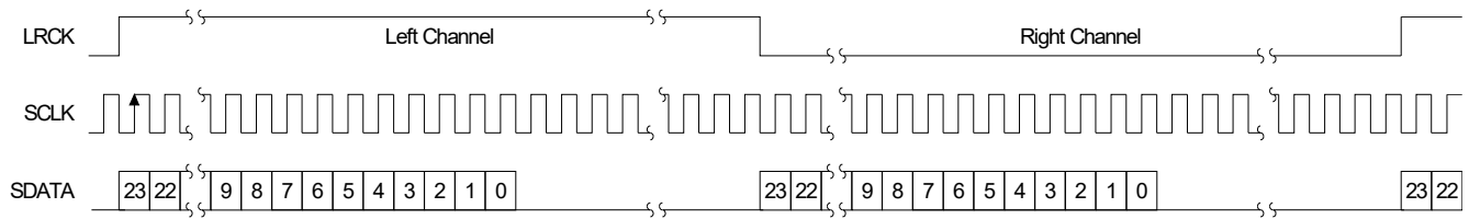
Figure 18. Left Justified Serial Audio Interface
