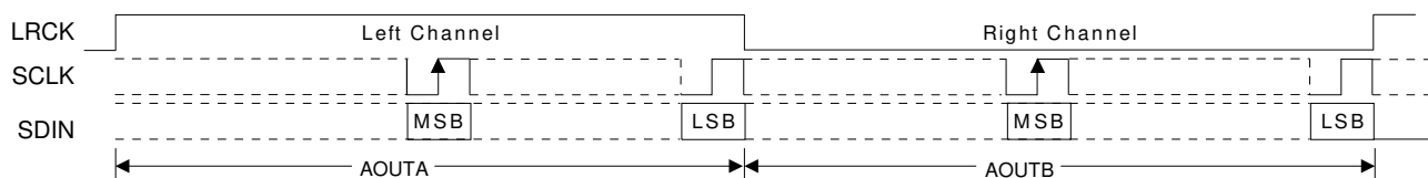
Figure 16. Right-Justified Format (DAC only)
