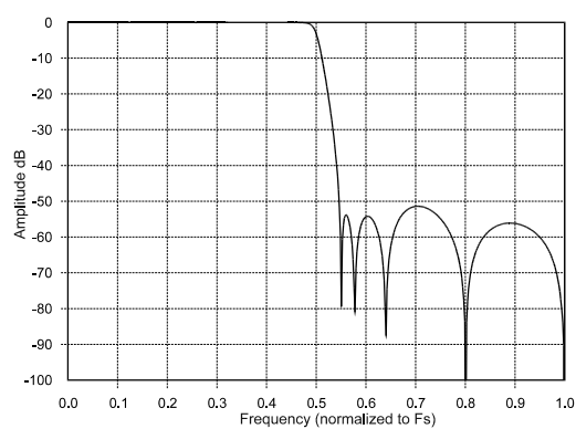
Figure 28. Stopband
