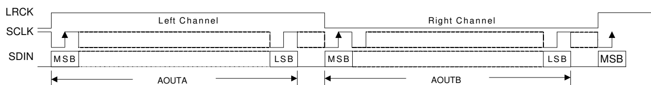
Figure 15. Left-Justified Format
