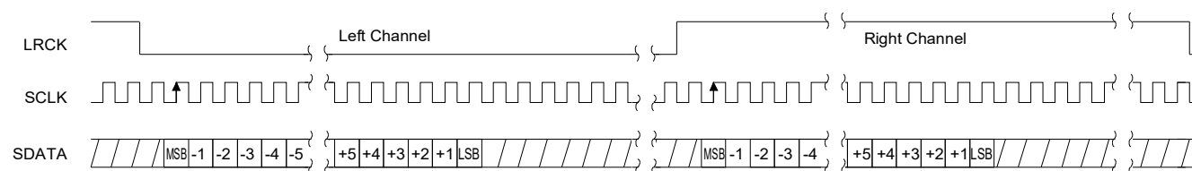
Figure 5. Format 1, I 2 S up to 24-Bit Data
