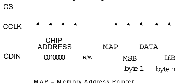
Figure 9. Control Port Timing, SPI mode
