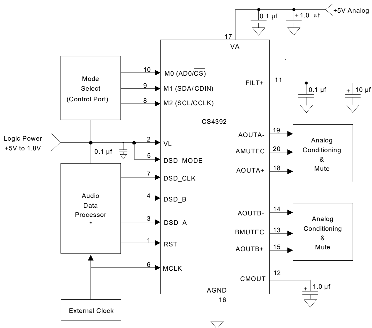
Figure 2. Typical Connection Diagram - DSD Mode
