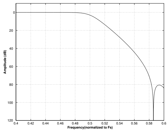
Figure 21. Double Speed (fast) Transition Band
