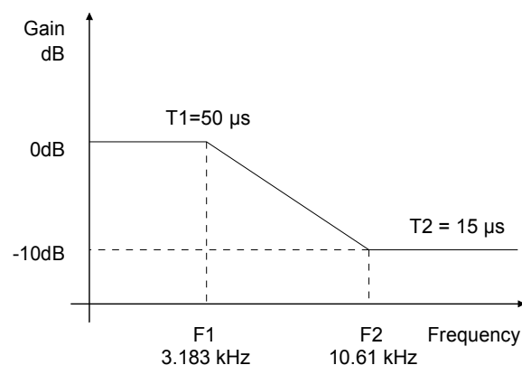
Figure 10. De-Emphasis Curve
