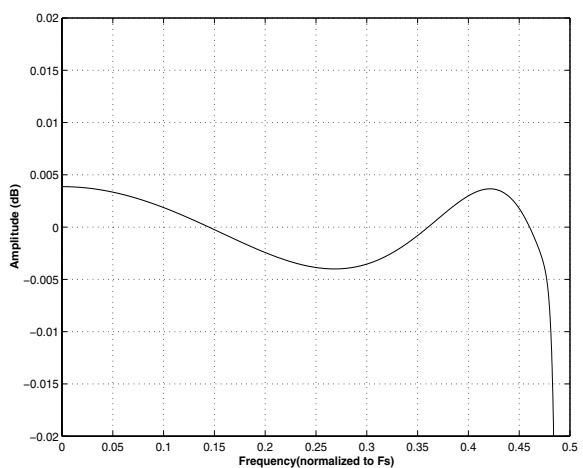
Figure 23. Single-Speed (fast) Passband Ripple
