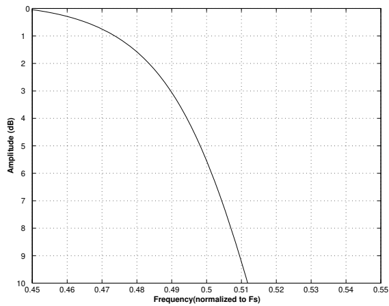
Figure 27. Quad-Speed (fast) Transition Band
