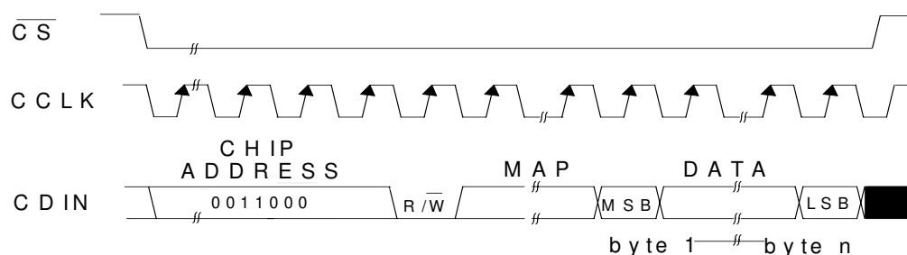
Figure 8. Control Port Timing, SPI Format
