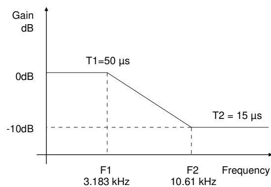
Figure 39. De-Emphasis Curve
