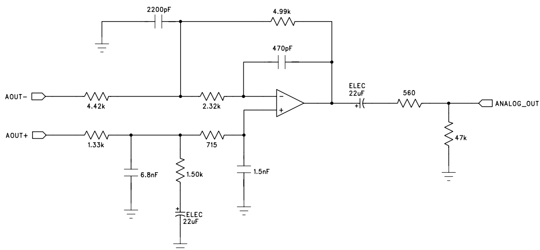
Figure 42. Recommended Output Filter
