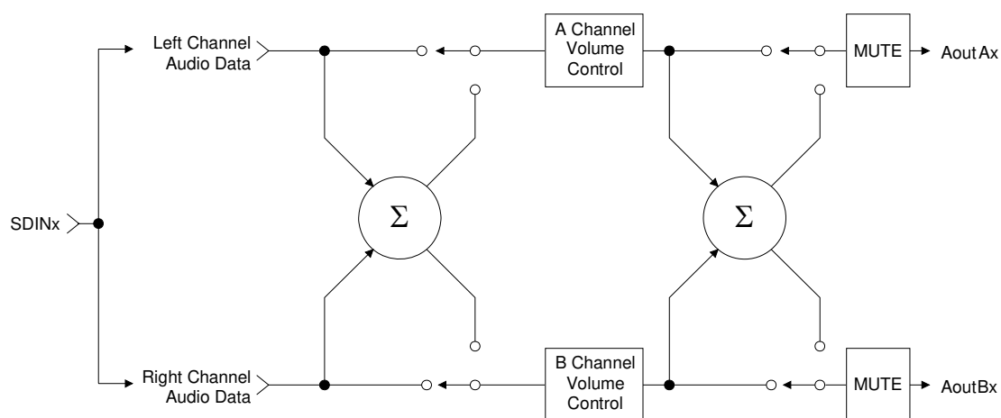
Figure 41. ATAPI Block Diagram (x = channel pair 1, 2, or 3)
