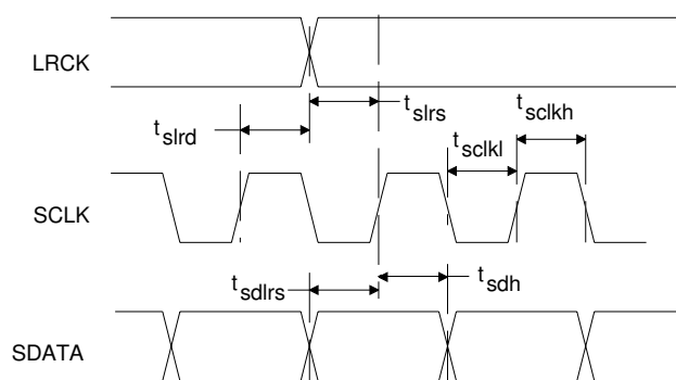
Figure 1. Serial Mode Input Timing
