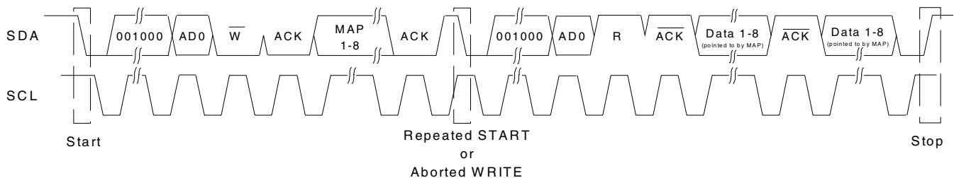
Figure 20. I²C Read
