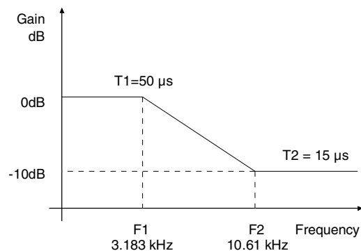
Figure 18. De-emphasis Curve
