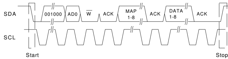
Figure 22. I²C Write
