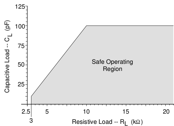
Figure 2. Maximum Loading
