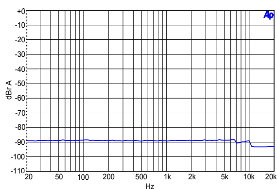
Figure 28. THD+N vs. Frequency (BRM)
