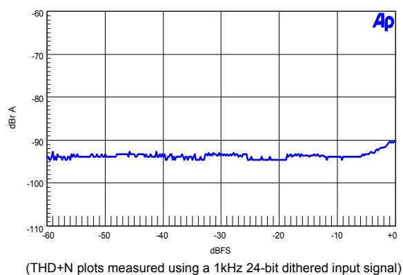
Figure 33. THD+N vs. Amplitude (HRM)
